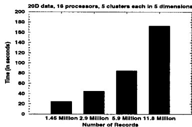
Figure 5. Scalability with database size
