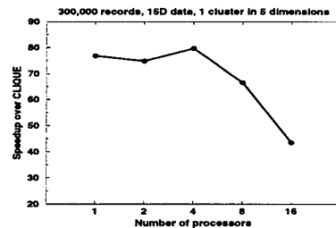
Figure 4. Speedup of pMAFIA over CLIQUE
