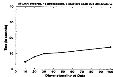
Figure 6. Scalability with Data Dimension
