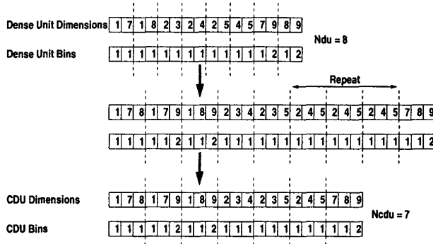
Figure 2. Building CDUs. (Dimension, k = 3 )
