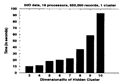
Figure 7. Scalability with Cluster Dimension
