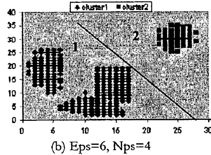
Figure 2 The different partitions resulting from running DBSCAN with different input parameter values.
