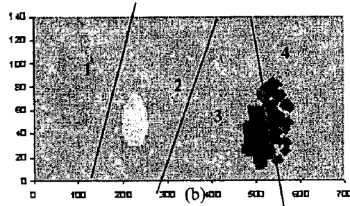
Figure 1 (a) A data set that consists of 3 three clusters, (b) The results from the application of K-means when we ask four clusters
