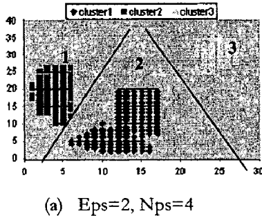
Figure 2 The different partitions resulting from running DBSCAN with different input parameter values.
