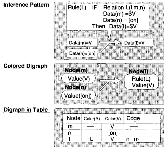
Fig. 4. Inference pattern, colored digraph and representation.
